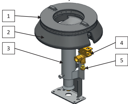
Figure 16. onstruction of the burner on the example of 7kW burner.
