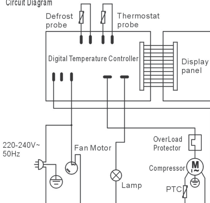
Circuit Diagram
