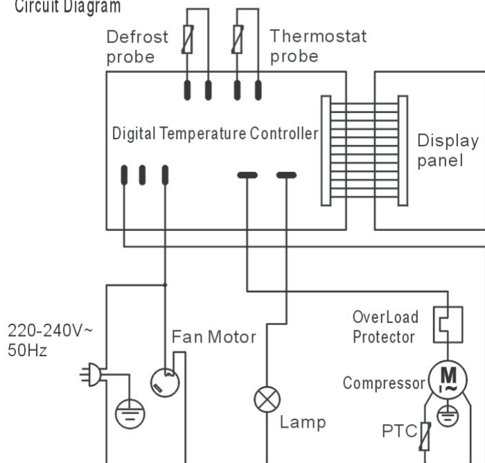
Circuit Diagram
