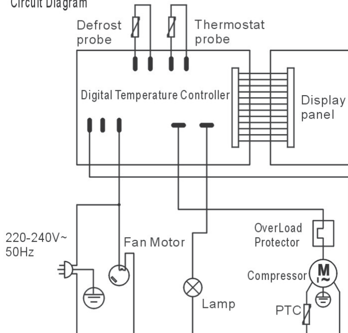
Circuit Diagram
